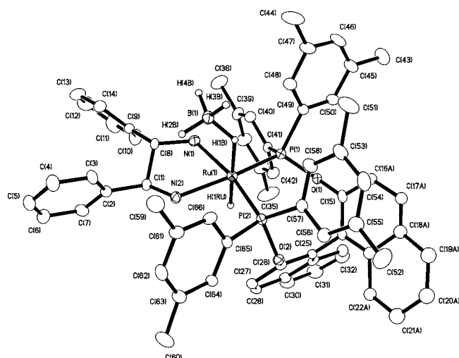
Figure 2. Structure of complex 4b .
