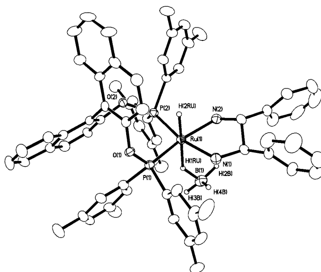
Figure 1. Structure of complex 3b . Only hydrogen of the hydride and borohydride ligands are shown.
